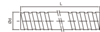
Fig 3.7.1 Screw Shaft Nominal Diameter
