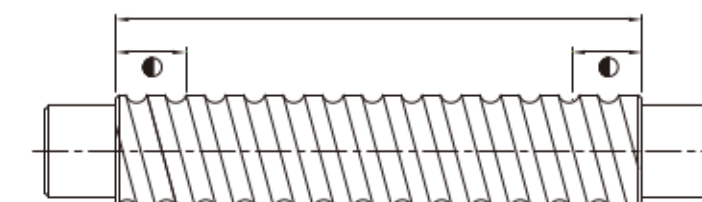
Fig 3.6.5 Harden Area
